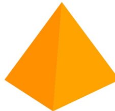
Square Pyramid
