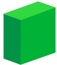
Cuboid
