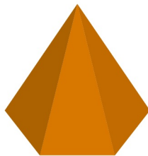
Hexagonal Pyramid
