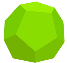
Dodecahedron
