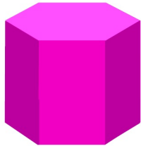
Hexagonal Prism
