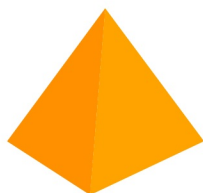
Square Pyramid
