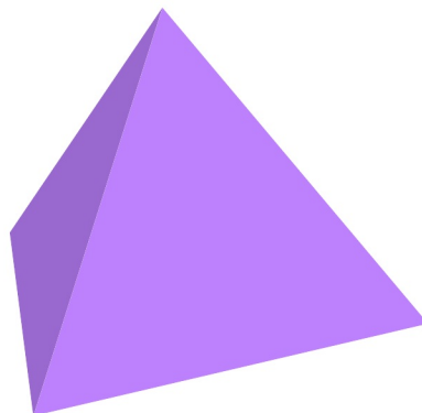
Tetrahedron
