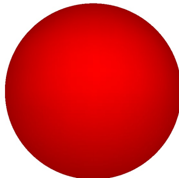
Sphere
