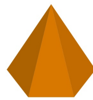
Hexagonal Pyramid
