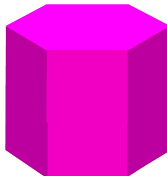
Hexagonal Prism
