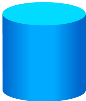
Cylinder
