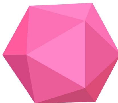
Icosahedron
