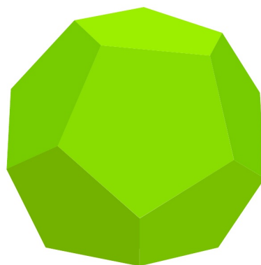
Dodecahedron
