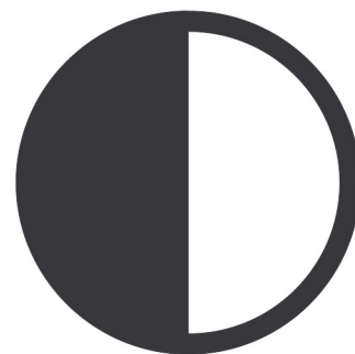
Waxing Quarter
