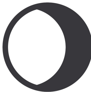
Waning Gibbous
