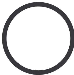
Full
