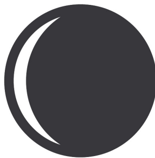
Old
