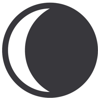
Waxing Gibbous
