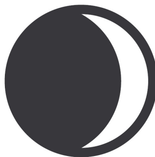
Waxing Crescent
