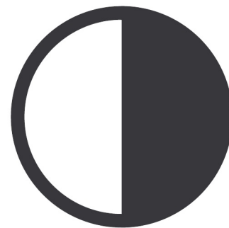
Waning Quarter
