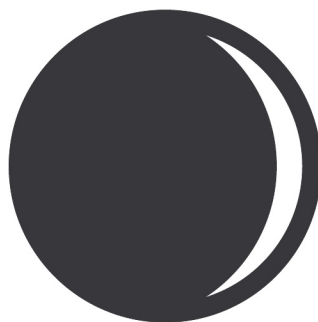
Young
